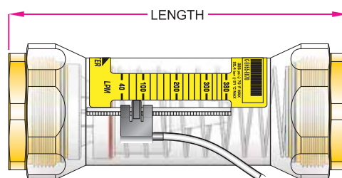
EZ-VIEW Flow Meter (with Flow-Alert Reed Switch)
